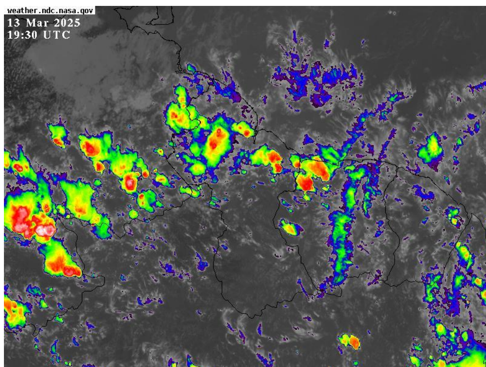
Infrared Satellite and Radar images valid 19:30 UTC (15:30hrs) Thursday, 13 March 2025.
