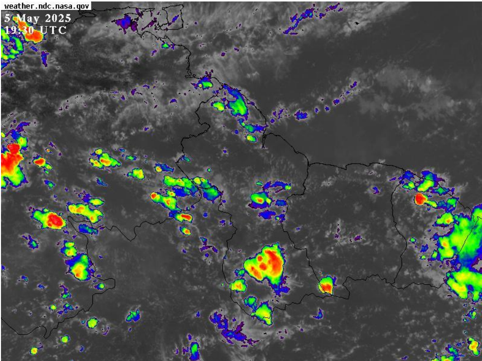
Infrared Satellite and Radar images valid 19:30 UTC (15:30hrs) Monday, 05 May 2025.
