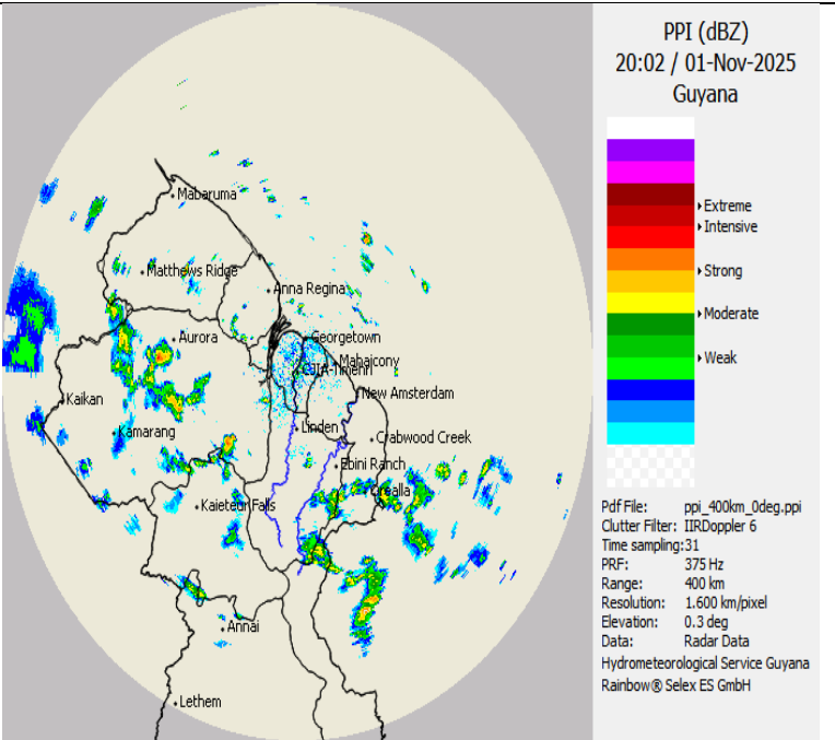
Radar image valid at 20:02 UTC (16:02hrs) Saturday, 01 November 2025.
