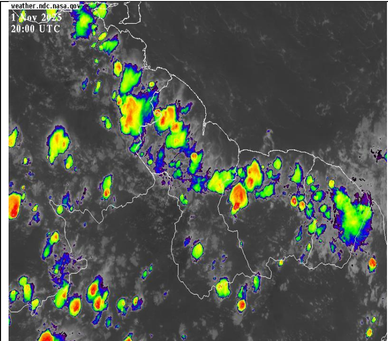
Infrared Satellite image valid at 20:00 UTC (16:00hrs) Saturday, 01 November 2025.
