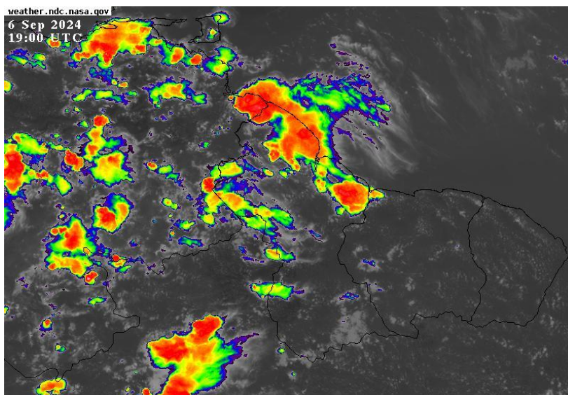
Infrared Satellite and Radar images valid 19:00 UTC (15:00hrs) Friday, 06 September 2024.
