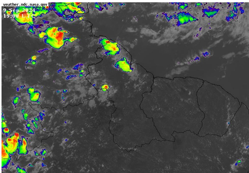
Infrared Satellite and Radar images valid 19:00 UTC (15:00hrs) Monday, 09 September 2024.
