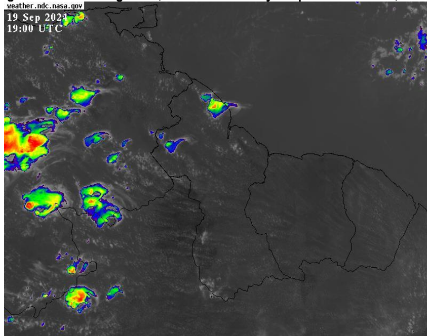
Infrared Satellite and Radar images valid 19:00 UTC (15:00hrs) Thursday, 19 September 2024.
