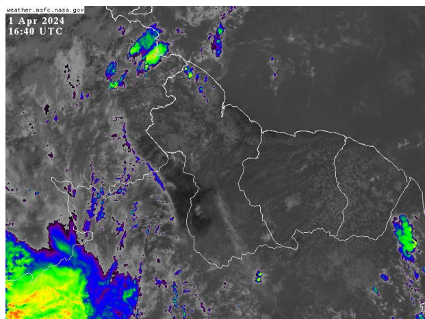
Infrared Satellite image valid 16:40 UTC (16:40 hrs) 01 April 2024.
