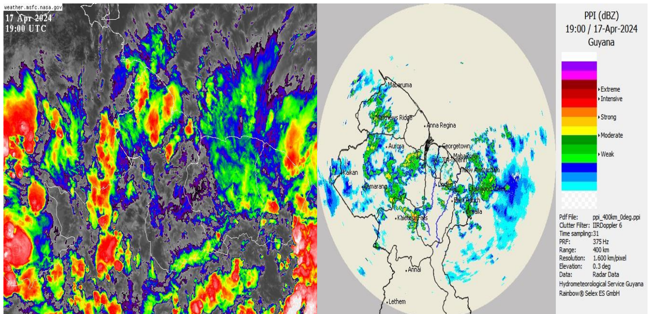
Infrared Satellite and Radar images valid at 19:00 UTC (15:00hrs) on 17 April 2024.
