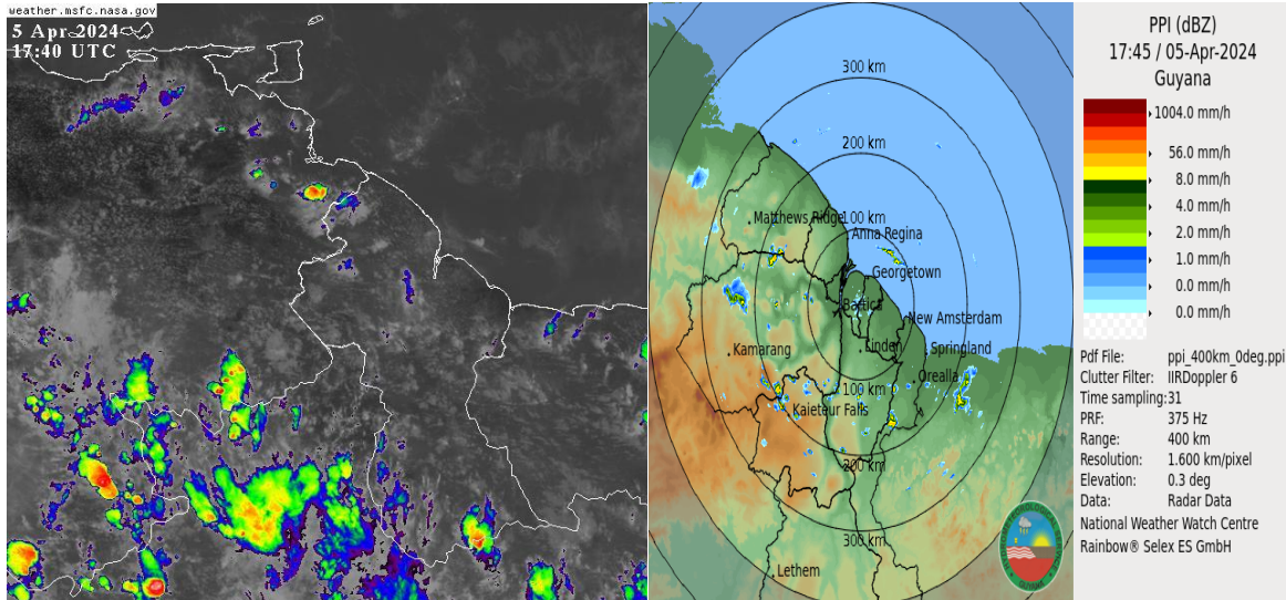
Infrared Satellite and Radar images valid 17:40 UTC (13:40 hrs) 05 April 2024.
