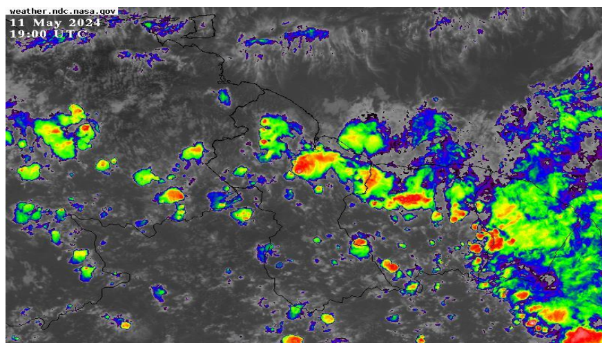
Infrared Satellite image valid at 19:00 UTC (15:00 hrs) Saturday, May 11, 2024
