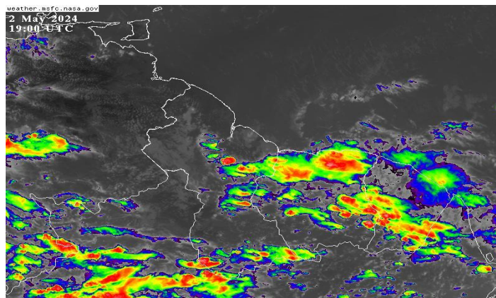
Infrared Satellite image valid at 19:00 UTC (15:00hrs) on 02 May 2024.
