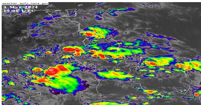
Infrared Satellite image valid 19:00 UTC (15:00 hrs) 03 May 2024.
